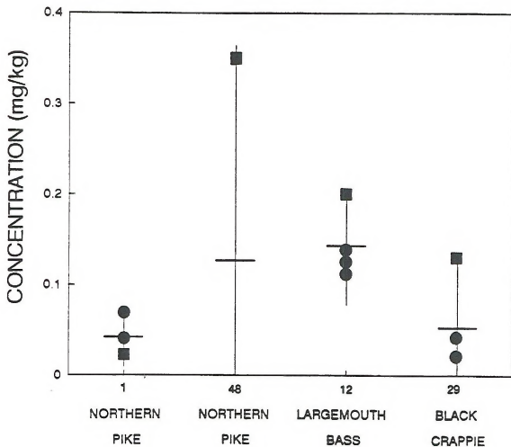
Figure 14. Comparison of replicate analyses from the same fish fillet. Squares represent the value of the initial determination while the circles represent mercury from randomly selected tissue samples. Mean concentration (horizontal bar) and 95% confidence intervals are shown for the four samples.
